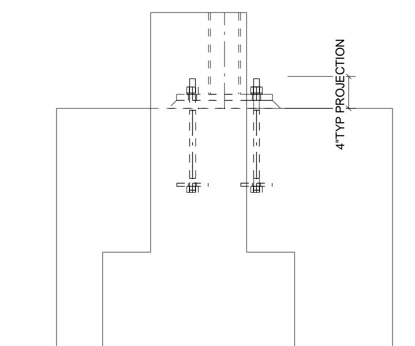
ANCHOR BOLT PROJECTION A - A
